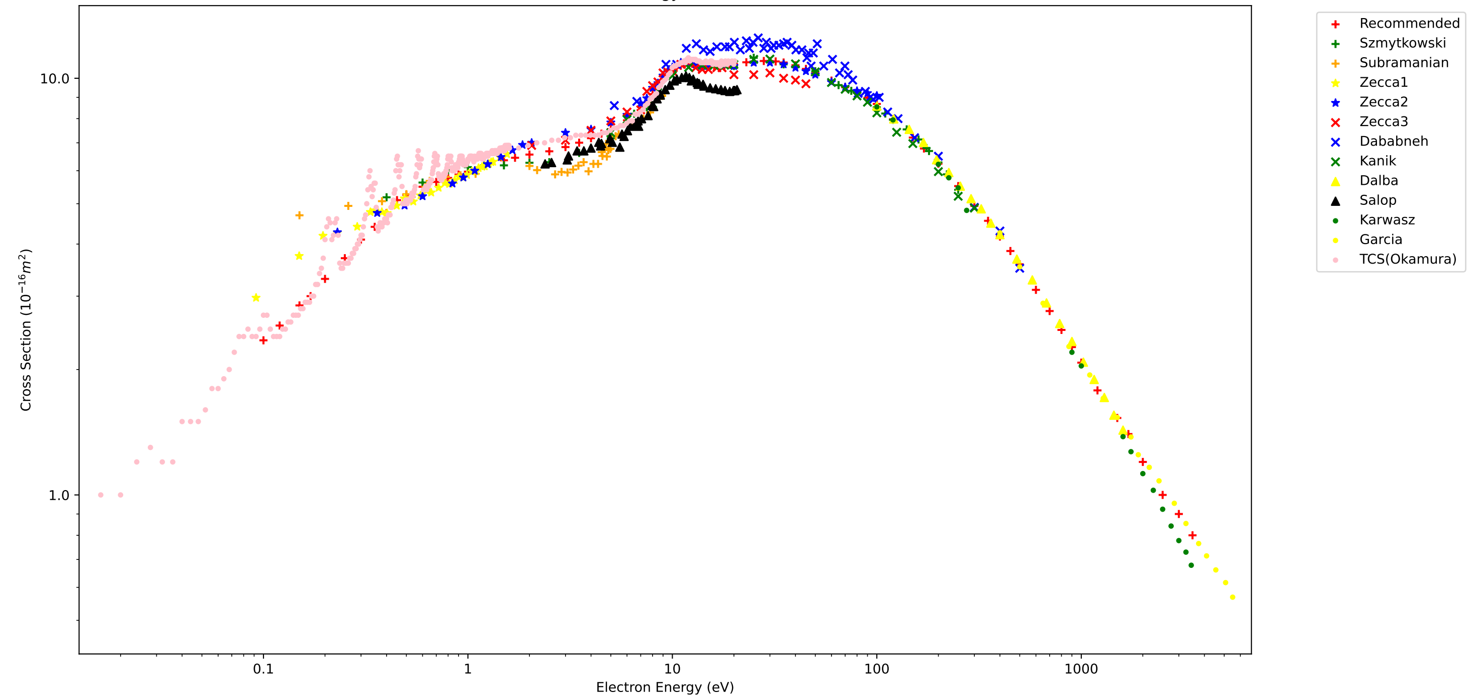
Cross Section vs. Energy for Different Studies
